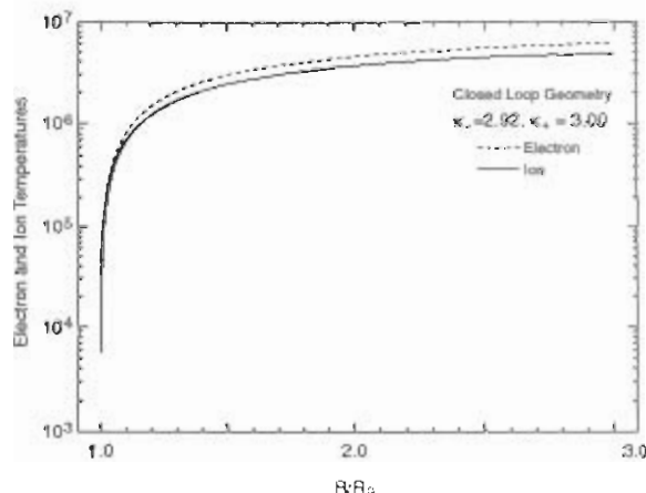
Figure 14. Electron and ion temperatures for solar coronal model using non-Maxwellian distributions and no heat deposition in the coronal [Scudder, 1992].
