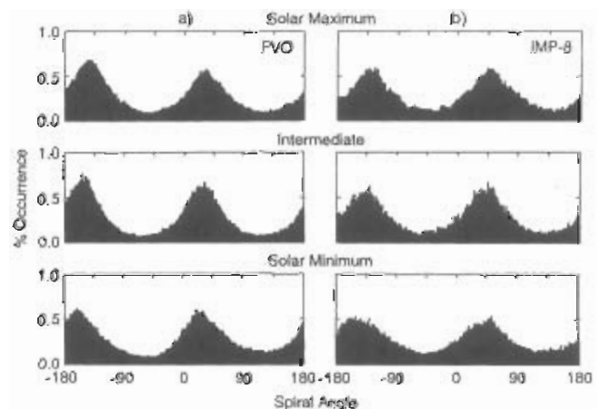
Figure 19. Histograms of the occurrence of various spiral angles in the Pioneer Venus 10-minute averages and the IMP-8 5-minute averages separated according to solar activity level [Luhmann et al. , 1993].
