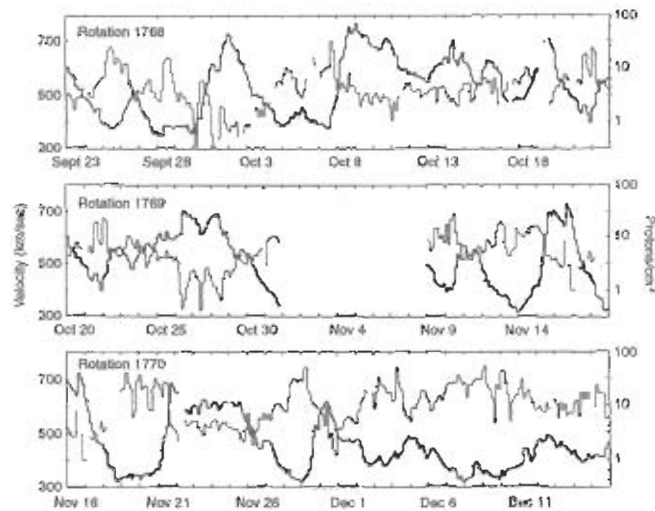
Figure 29. Solar wind velocity (dark line) and density (light line) measured by Mariner 2 on three successive solar rotations. Adapted from Hundhausen [1995].
