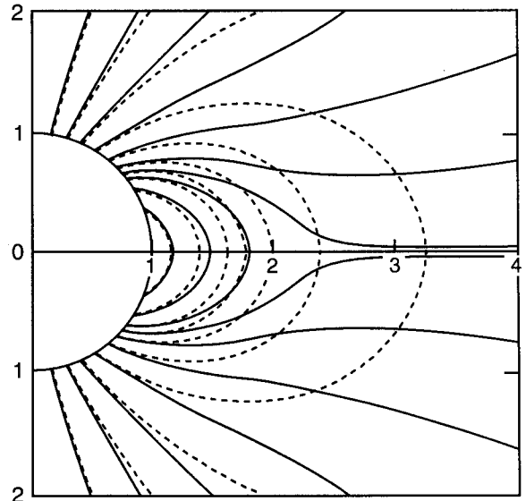
Figure 16. Coronal magnetic field in the Pneumann and Kopp [1971] isothermal solar wind solution. Dashed field lines show the magnetic field lines of a dipole for comparison.
