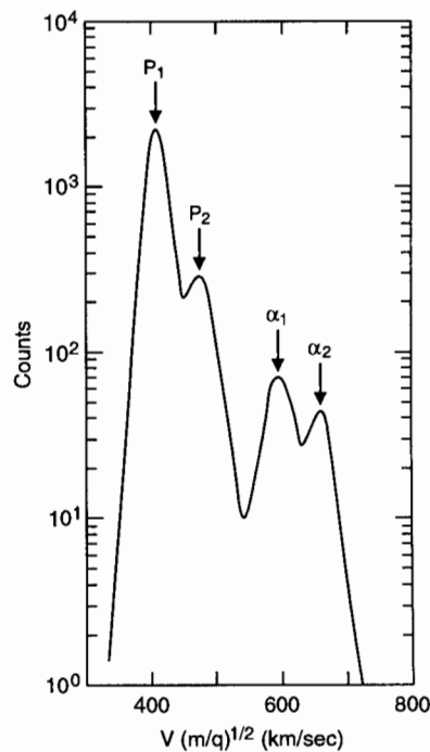
Figure 3. Unnormalized energy per charge spectrum of the solar ion population at a time when interpenetrating proton and alpha particles are present. These two alpha particles beams have the same velocities along the magnetic field as the two proton beams. Adapted from Asbridge et al., [1974].
