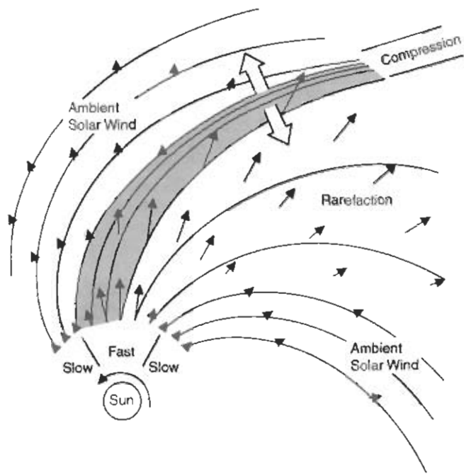
Figure 28. The collision of a fast stream with a slow stream to produce a corotating interaction. Adapted from Pizzo [1985].
