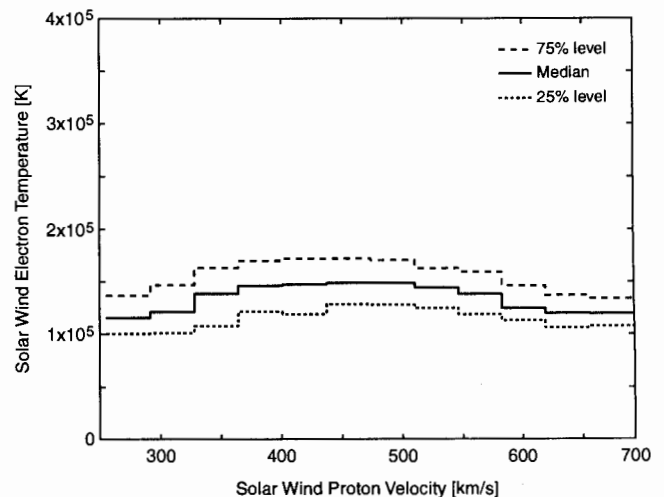
Figure 11. The temperature of solar wind electrons as a function of the solar wind velocity. The median and quartiles are shown. Adapted from Newbury [2000].
