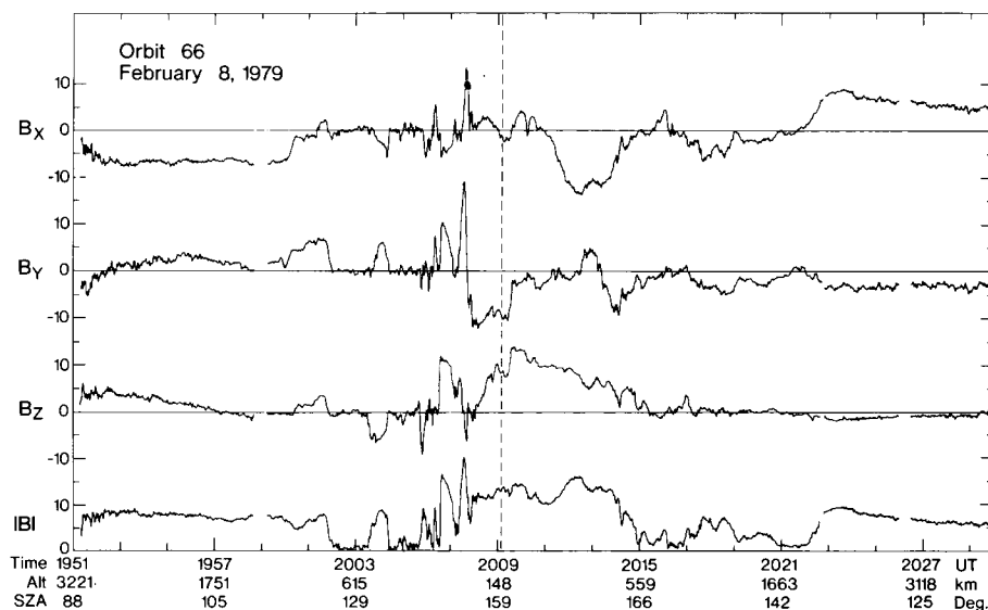
Fig. 2. High-resolution (two samples per second) magnetic field measurements for orbit 66. The dashed line designates periapsis. Vector components are in a coordinate system close to solar ecliptic coordinates. Units are nanoteslas.
