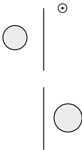
Impulsive Penetration
