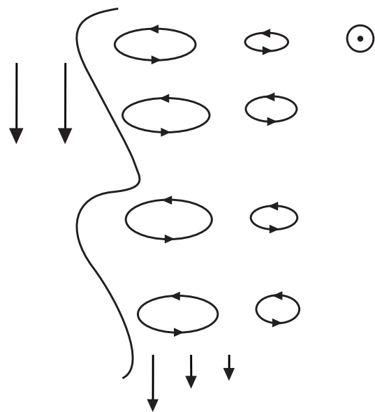
Kelvin-Helmholtz Instability
