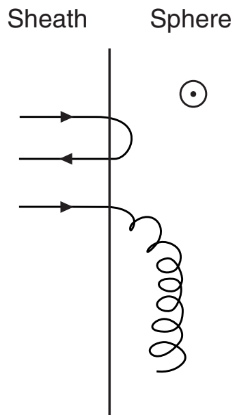
Diffusive Entry
