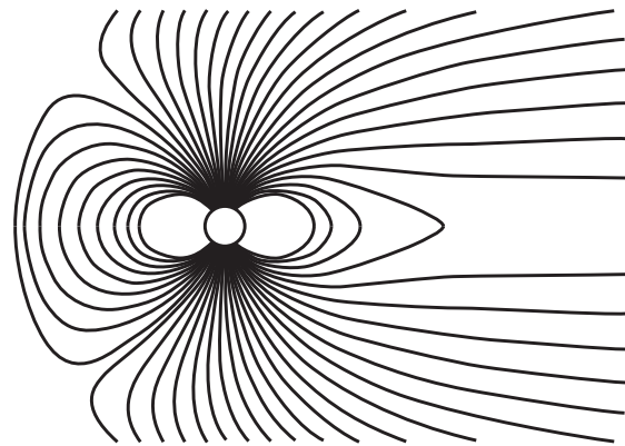
Empirical Magnetosphere
