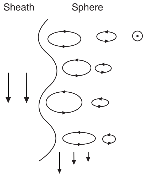
Boundary Oscillation
